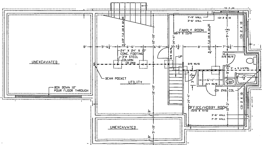
FOUNDATION & LOWER LEVEL PLAN
